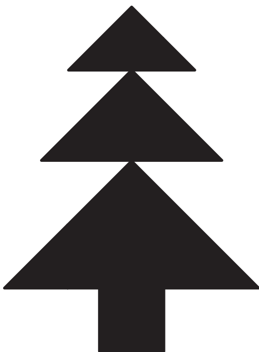
TREE
